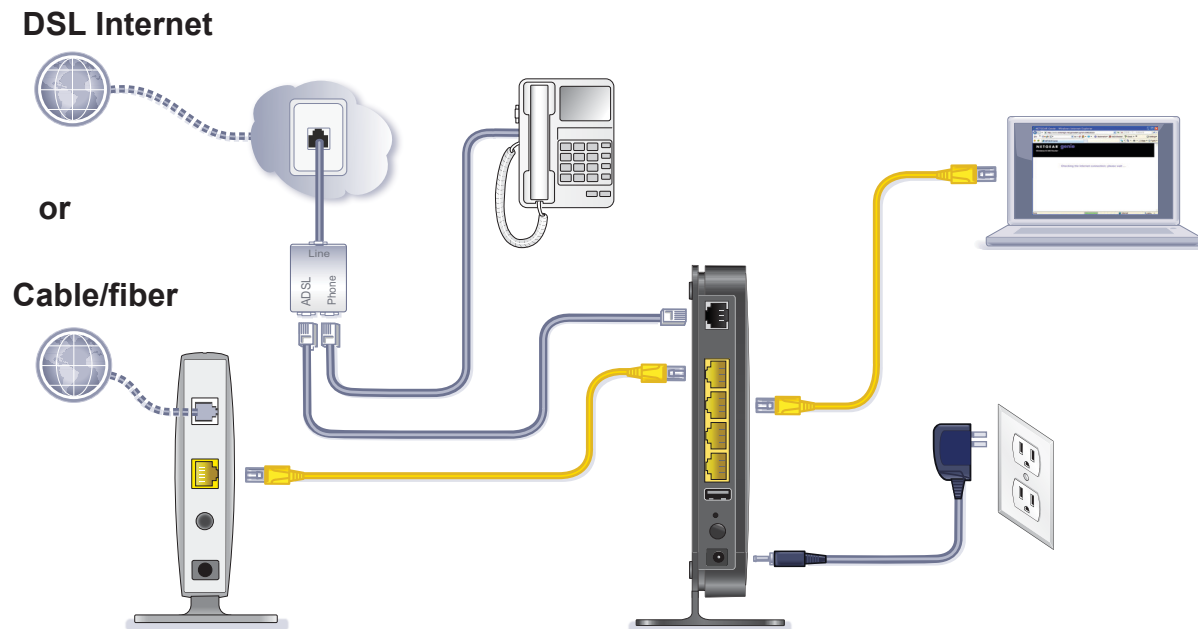
Figure 7. Cable connections
