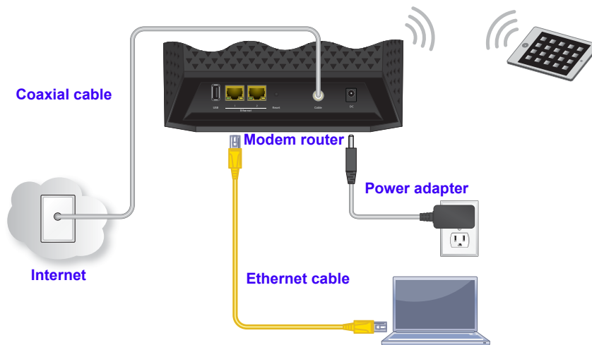
Figure 3. Modem router in a simple network
