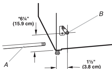
A. 1/2" NPT gas supply line B. 3/8" NPT dryer pipe
