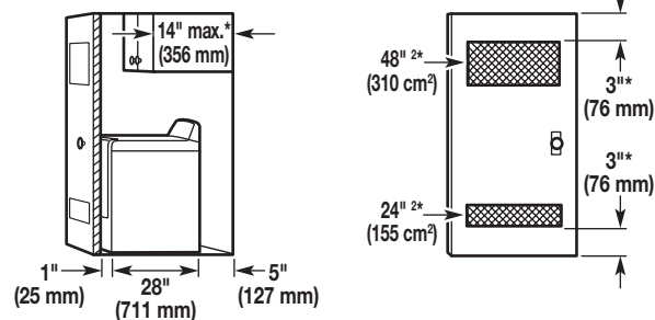
Side view - closet or confined area (Dryer with flat back)
