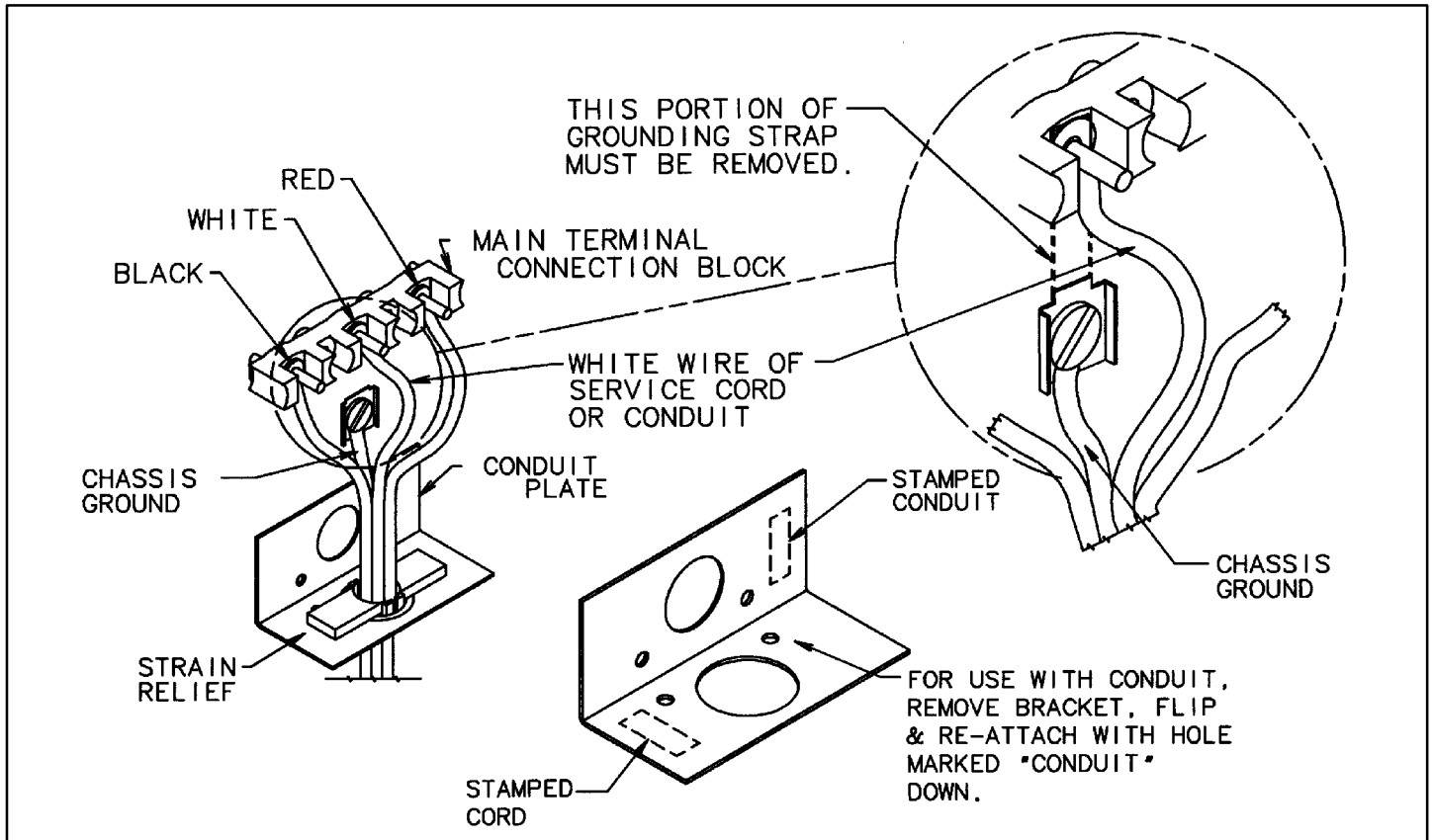
FIGURE 8 ACCEPTABLE 4-WIRE PLUG INSTALLATION
