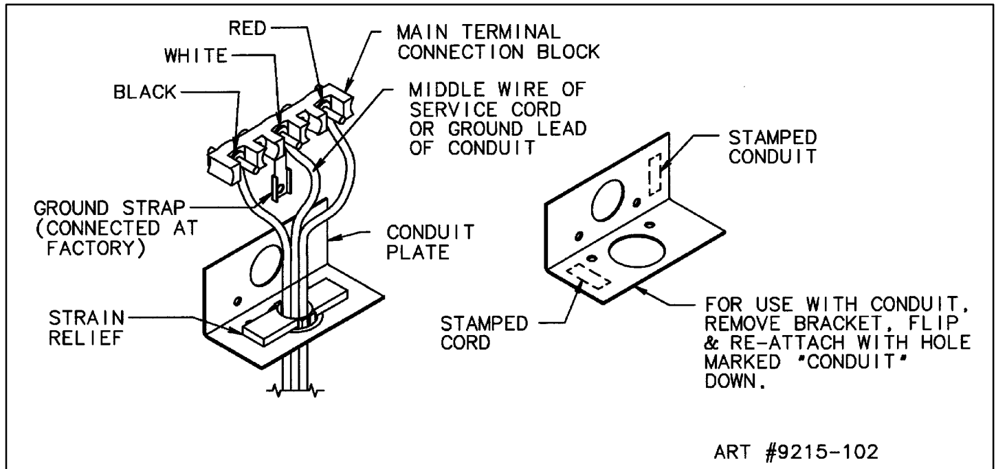
FIGURE 7 ACCEPTABLE 3-WIRE PLUG INSTALLATION
