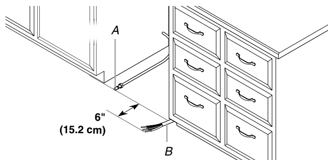
A. Water supply line B. Direct wire
