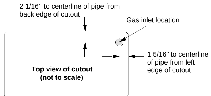
Cooktop supplied with 1/2" NPT female inlet on regulator
