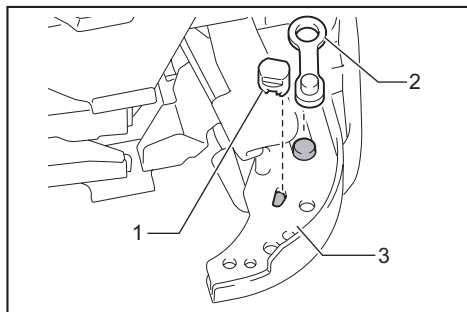
► 1. Cutter A 2. Link arm A 3. Arm plate A
