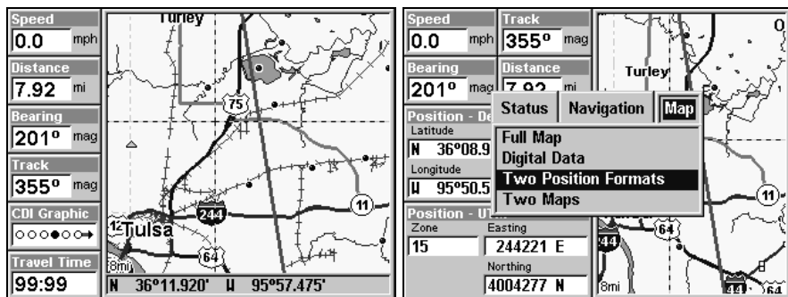
GlobalMap Digital Data page (left) and Two Position Formats page (right).
