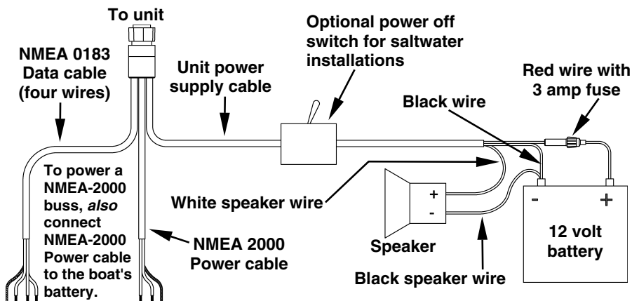
Power and optional speaker connections for the GlobalMap units covered in this manual.
