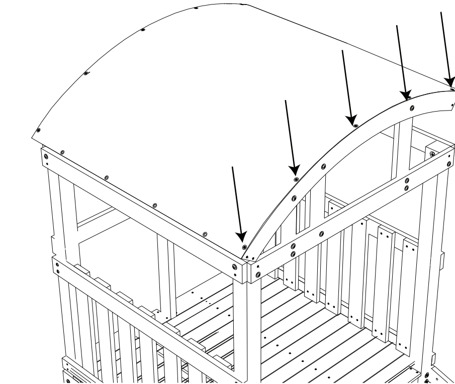
Step 71: Attach the Tarp Roof to the Roof Rafters using (5) Screws (SW16).
