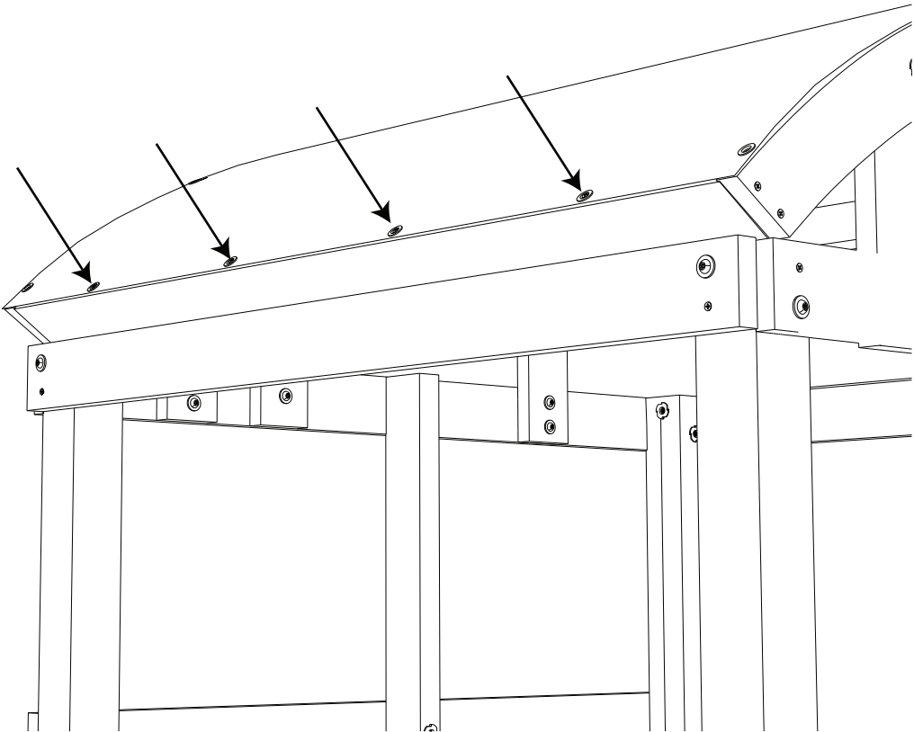
Step 73: Attach the Tarp Roof to the Roof Brace (F13) using (4) Screws (SW16).
