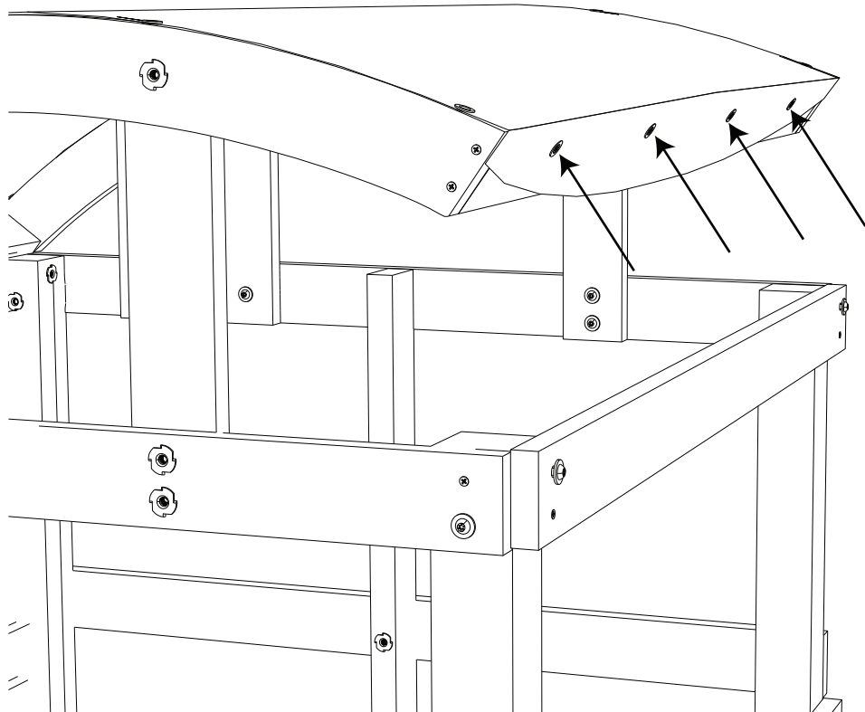
Step 72: Attach the Tarp Roof to the Roof Brace (F13) using (4) Screws (SW16).
