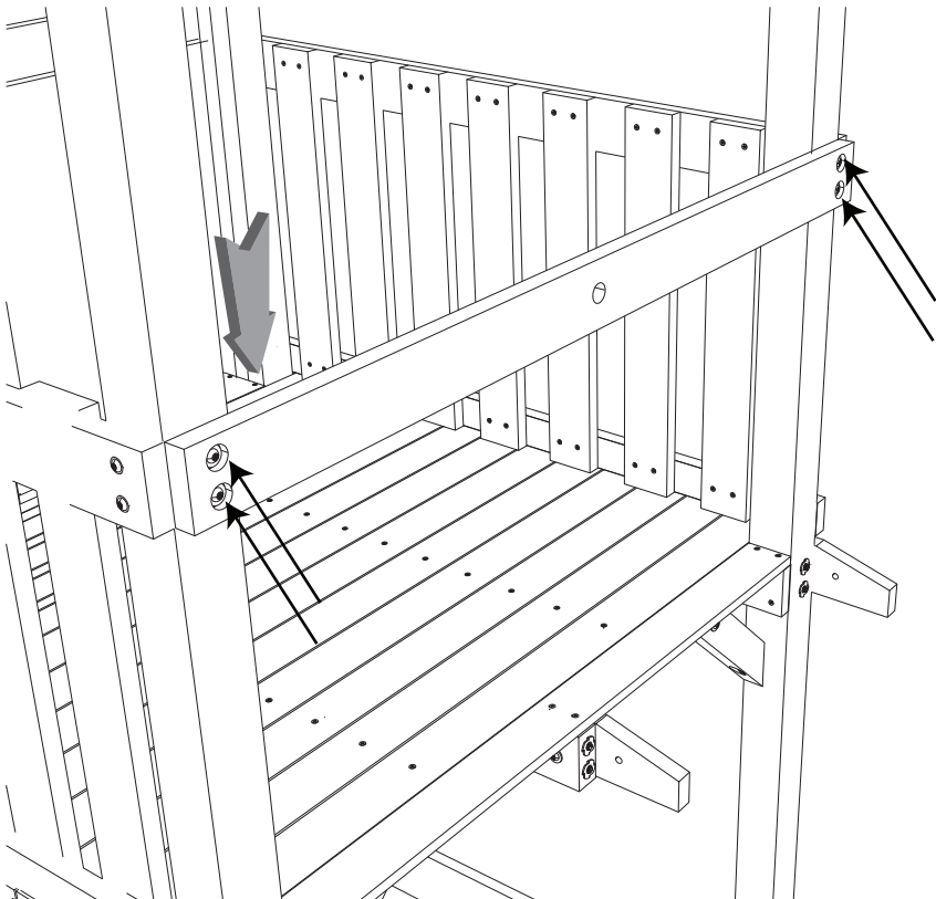
Step 74: Attach (1) Wall Rail (K08) to Tower Legs 2 and 1 using (4) Screws (M8SW60). Ensure the Wall Rail (K08) is flush with the tops of Handrails (F09).
