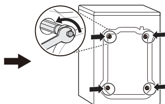
Unpacking and removing shipping bolts
