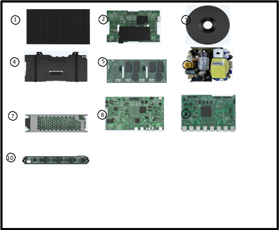
Figure 2.2 Major components of LUPA098 LED panel assembly
