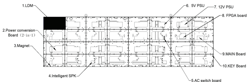
Figure 2.1 Major components placement for LUPA098
