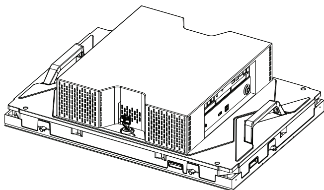
Back Cover for LDAA025-MD (IMB Built-in Back Cover)
