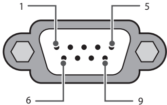
RS-232C (Serial port)
