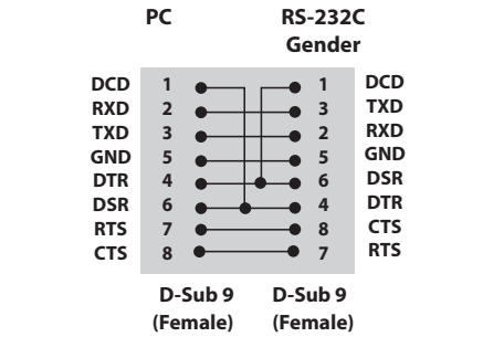
8-Wire Configurations (Standard RS-232C cable)
