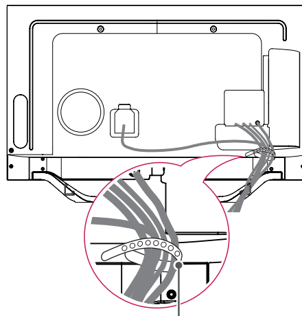
Cable Holder
