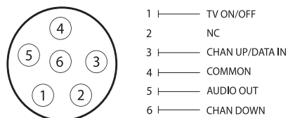
Pillow Speaker Interface Pinout
