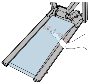
Figure 4-2. Treadbelt Tension Check
