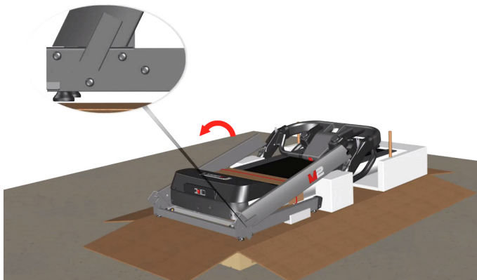
Figure 2-15. Unfold Frame Uprights – Finish
