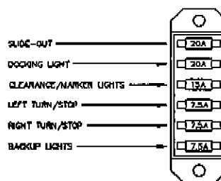
Exterior Light Fuse Box (Lance Only)
