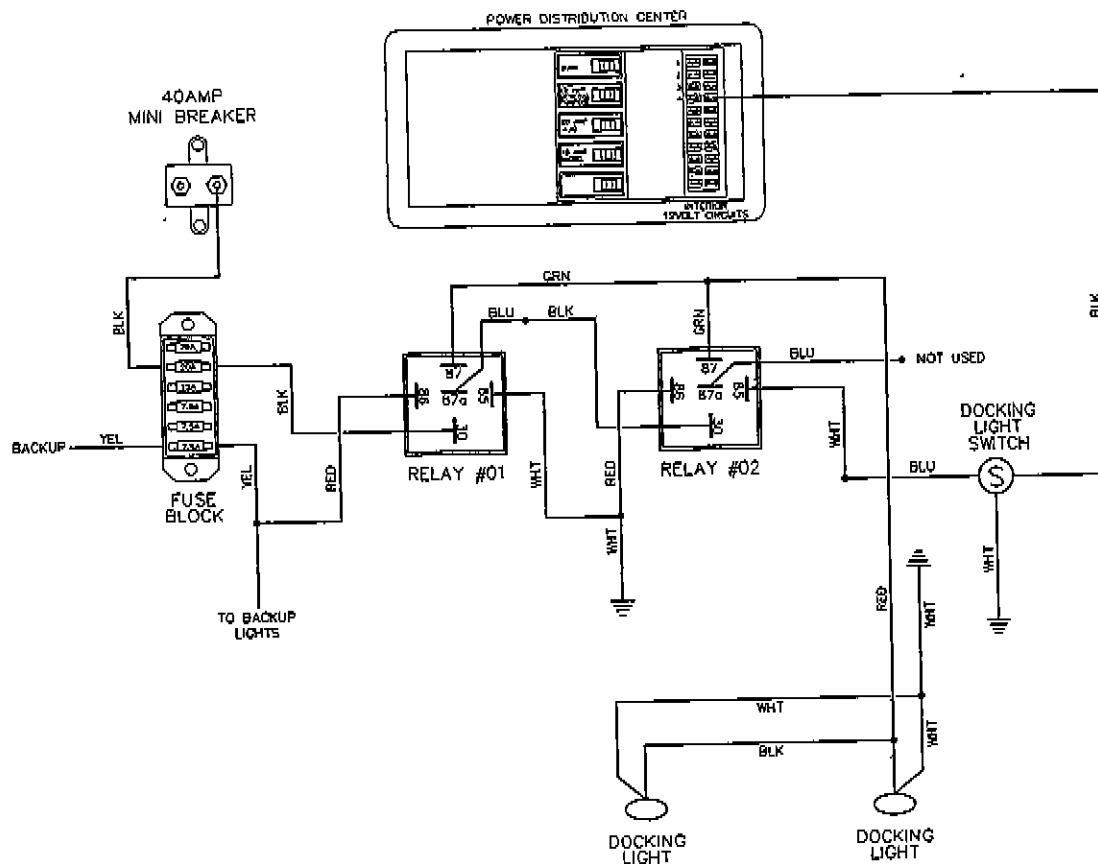
Docking Light Relay Wiring Diagram
