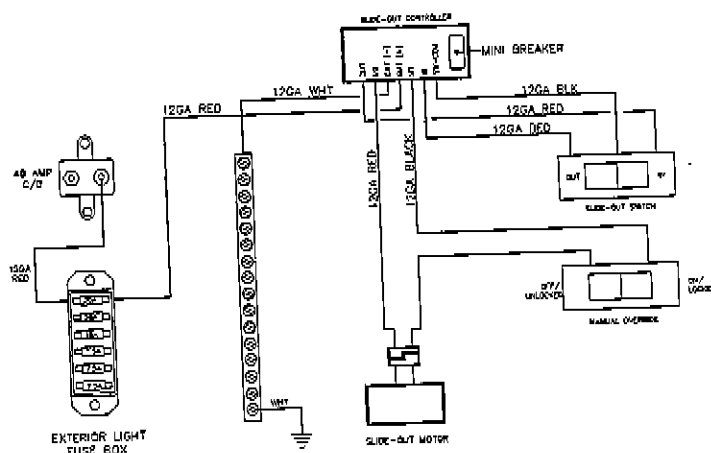
Slide-Out System Electrical Diagram
