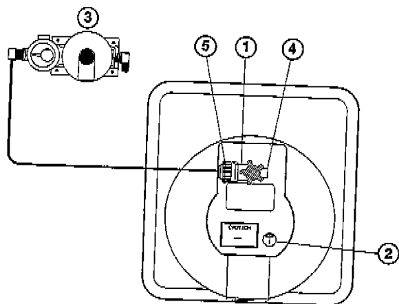
Single Laydown LPG Tank Installation
