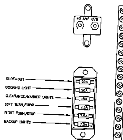
Exterior Light Fuse Box (Lance Only)
