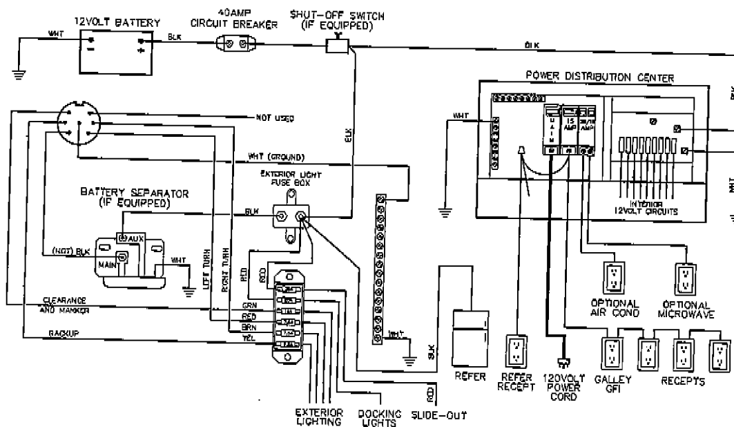
Electrical System Wiring Diagram (Typical)
