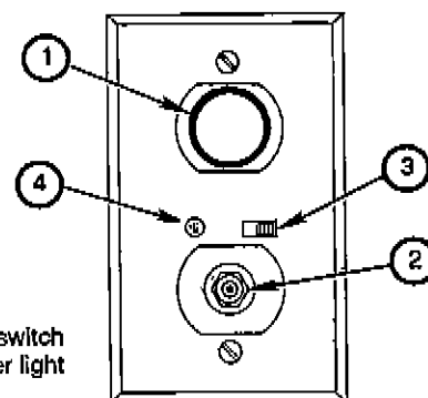
12-volt, Cable TV, Antenna Outlet
