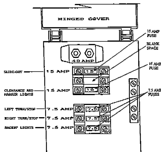
Exterior Light Fuse Box
