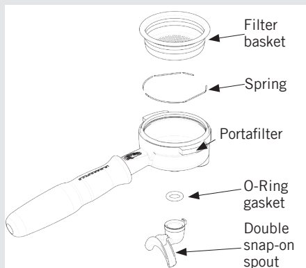
Figure 3 - Portafilter
