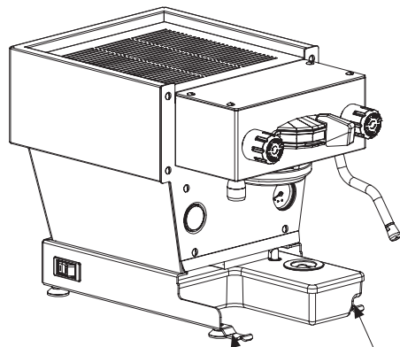
Alignment grooves
