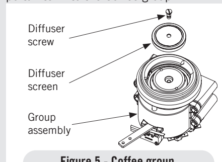
Figure 5 - Coffee group
