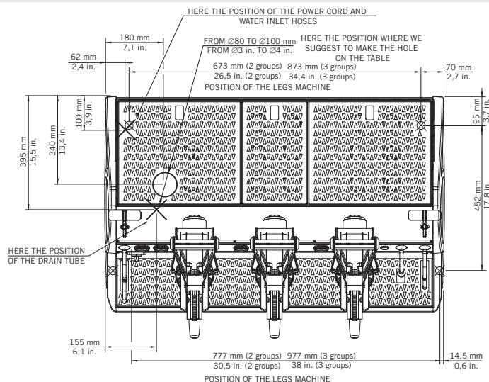
Fig. 3 - Installation guide
