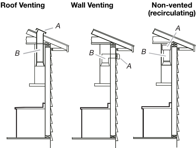
A. Roof cap B. 6" (15.2 cm) round vent A. Wall cap B. 6" (15.2 cm) round vent A. Deflector B. 6" (15.2 cm) round vent
