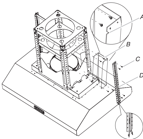
A. Notch in support B. Support C. 4.2 x 8 mm screws D. Vertical duct cover support
