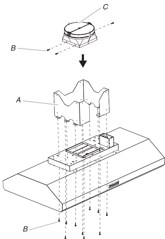
A. Lower support bracket B. 4.2 x 8 mm mounting screws C. Transition piece
