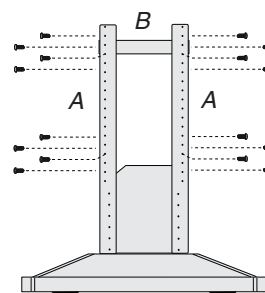
A. Vertical supports B. Horizontal support
