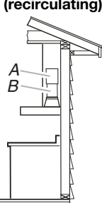
A. Diverter B. 6" (15.2 cm) round vent extension
