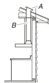
A. Roof cap B. 6" (15.2 cm) round vent
