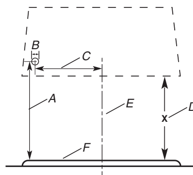
A. Distance "X" + 3" (7.6 cm) B. 1 \frac{1}{4} " (3.2 cm) diameter C. 7 \frac{1}{4} " (18.4 cm) for 30" (76.2 cm) models 8 \frac{1}{4} " (21.0 cm) for 36" (91.4 cm) models D. Distance "X" (30" [76.2 cm] min, suggested 36" [91.4 cm] max) E. Vertical centerline F. Cooking surface
