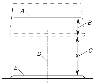
A. Horizontal line B. 11 \frac{3}{8} " (28.9 cm) C. Distance "X" (30" [76.2 cm] min, suggested 36" [91.4 cm] max) D. Vertical centerline E. Cooking surface
