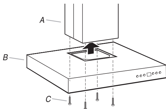
A. Chimney support B. Hood C. Bolts
