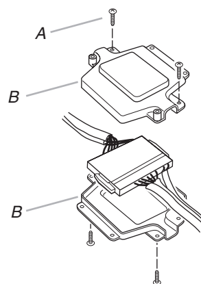
A. Screws B. Connector box half
