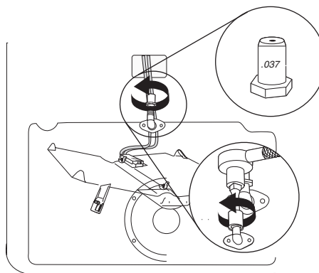
A. Number 0.037 LP gas broil burner orifice hood
