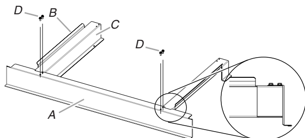
A. Bottom vent B. Spacer bar flange C. Spacer bars D. \frac{3}{8} " hex washer head screws
