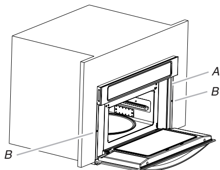
A. Mounting rail B. Two screws
