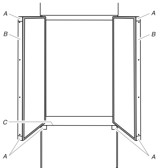
A. Corner caps B. Refrigerator door trims C. Freezer drawer trim
