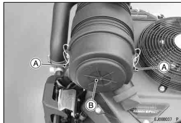
A. Retaining Clamps
