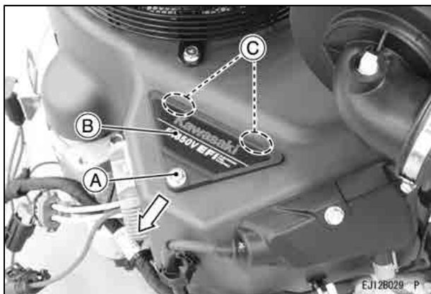
A. Cleanout Cover Bolt B. Cleanout Cover C. Tabs
