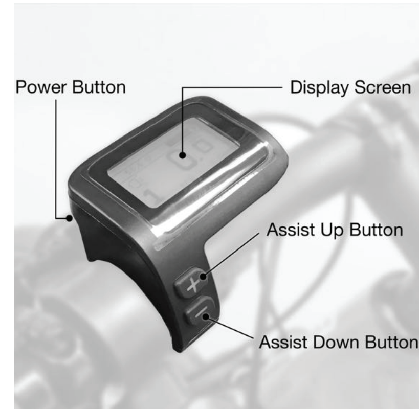
Fig. 5 - Buttons on the Advanced Matrix Display
