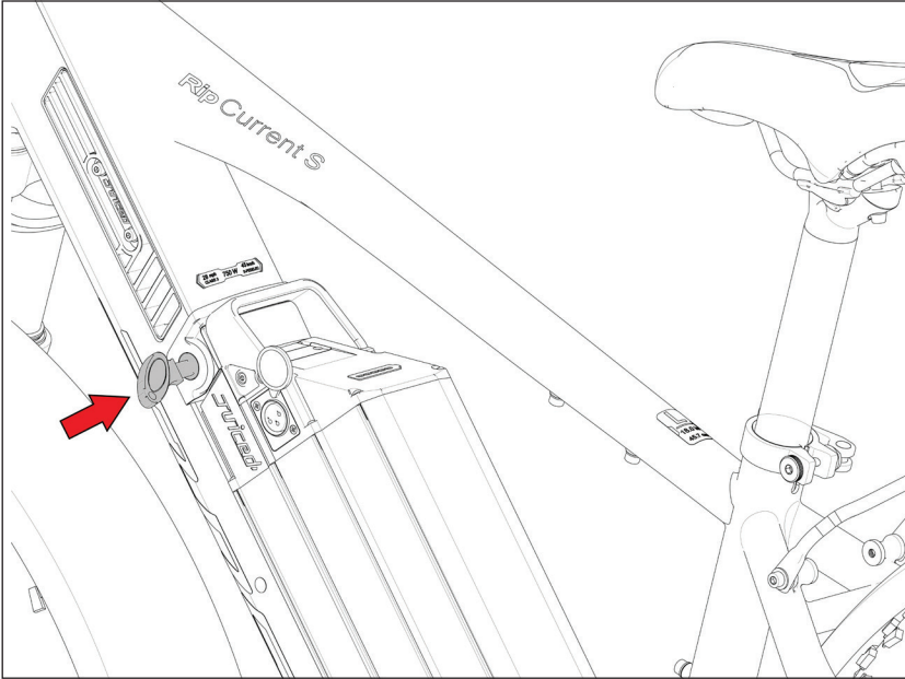
Fig. 10 - Removing Battery Pack
