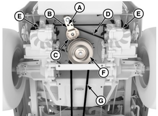
Components Viewed from Bottom
