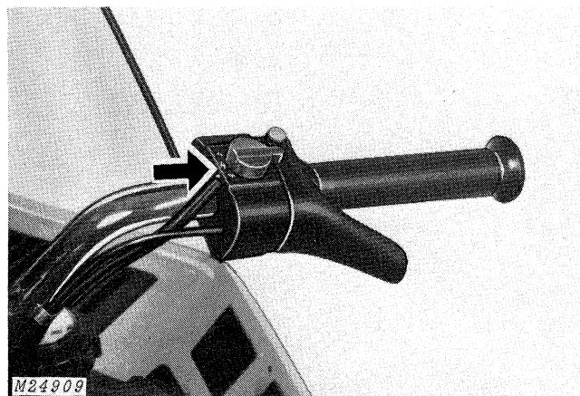
Normal Choke
