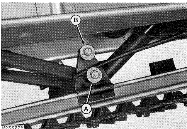
A—Bottom Position
