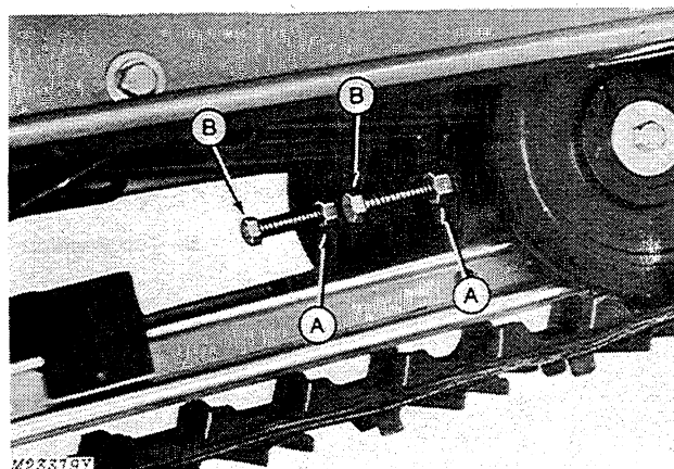
B—Adjusting Screws
