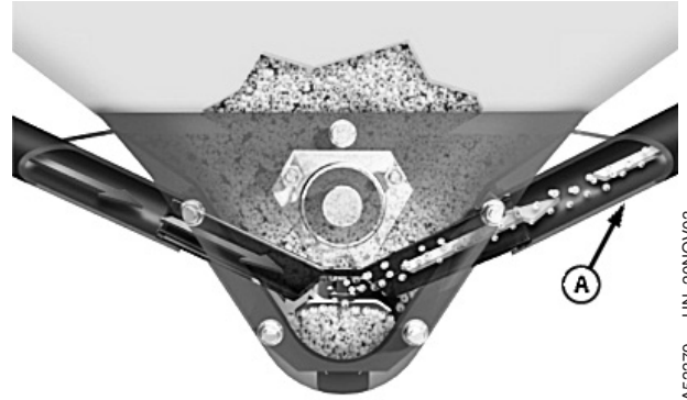
A—Delivery Hose
