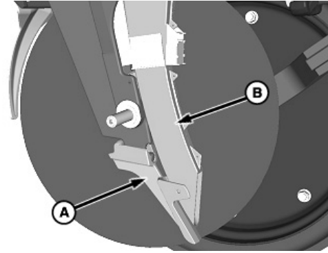
A—Seed Tube Guard B—Seed Tube
