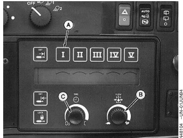
8000, 9000 Series
