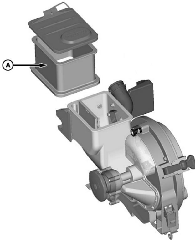
A—Extension
