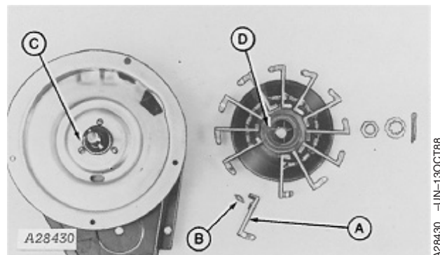
A—Pick-Up Finger B—Spring C—Notch in Bearing D—Projection on Cam
