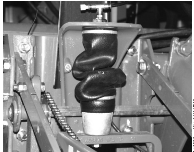
Improperly Rolled Air Bag
