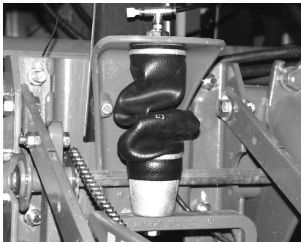
Improperly Rolled Air Bag
