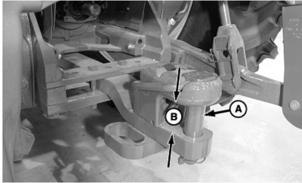
A—Drawbar Pin
