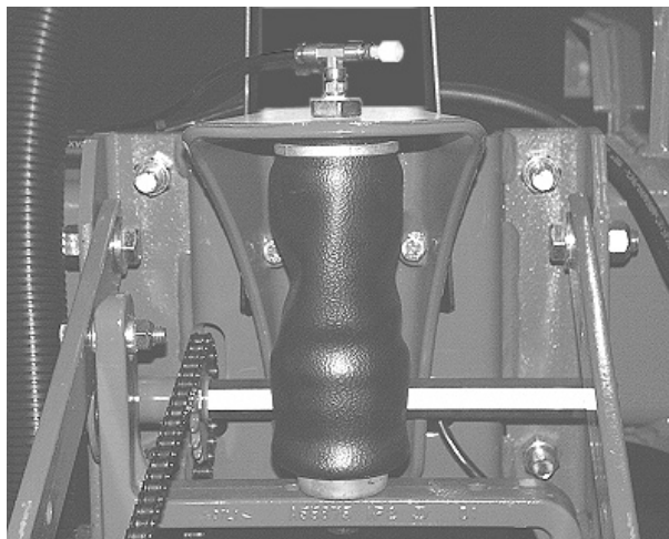
Properly Rolled Air Bag
