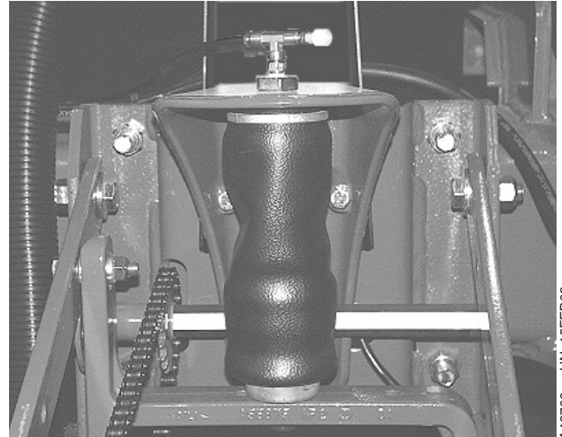
Properly Rolled Air Bag
