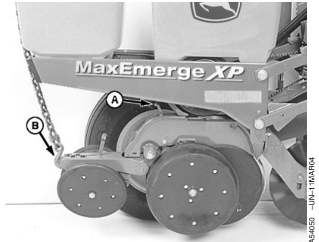
A—Depth-Adjusting Handle B—Chain
