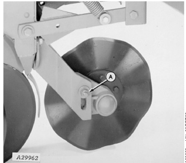
A—Cap Screw
