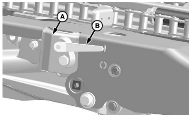
A—StalkMaster™ 切碎型齿轮箱 B—结合/分离手柄
