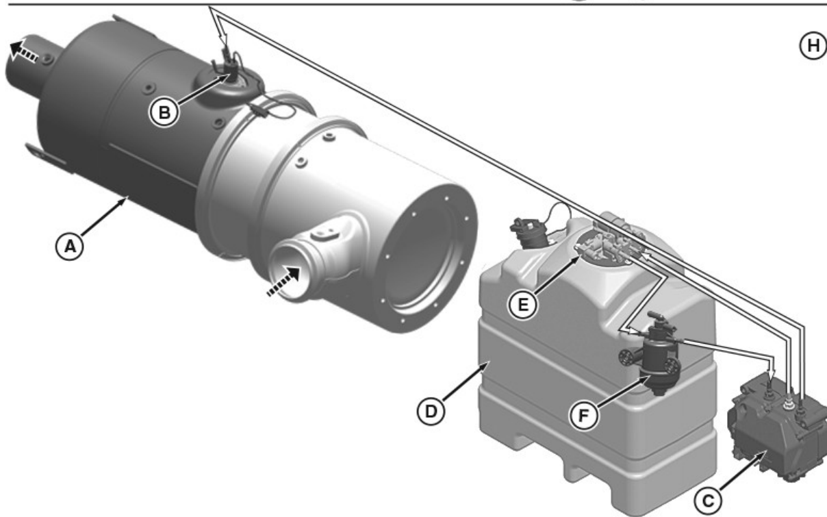
SCR-System
