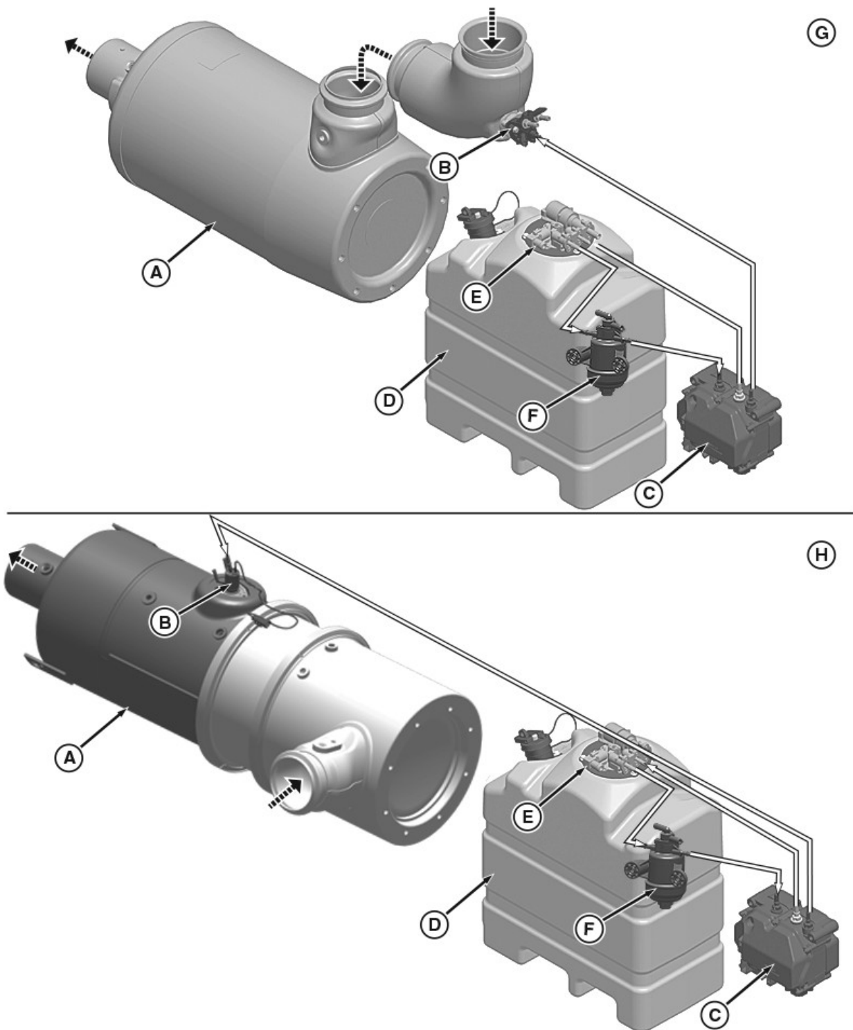
System SCR
