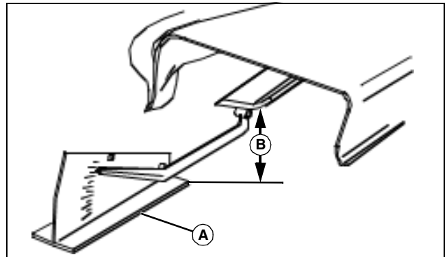
Picture Note: A convenient leveling gauge (A) (AM130907) is available from your dealer.
