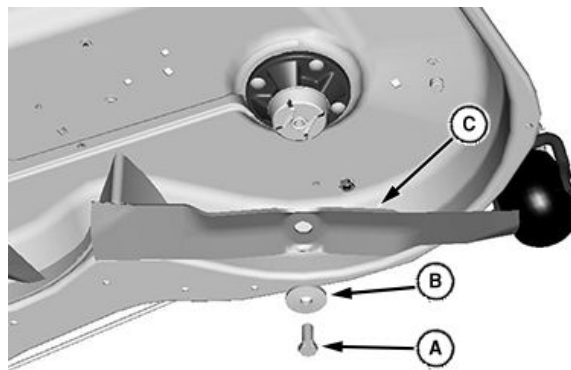
A—Perno B—Arandela
