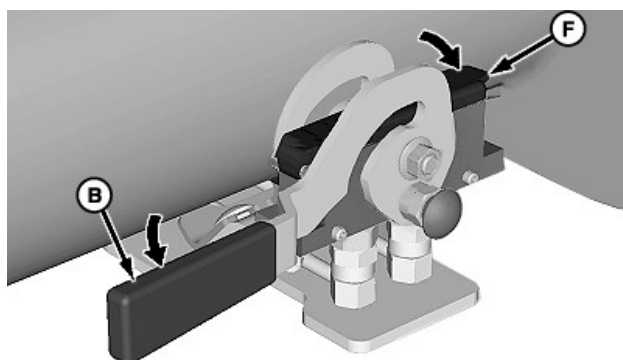
Grapple Attachment Shown
