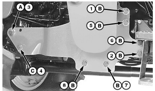
Torque Sequence (left-hand side shown)
