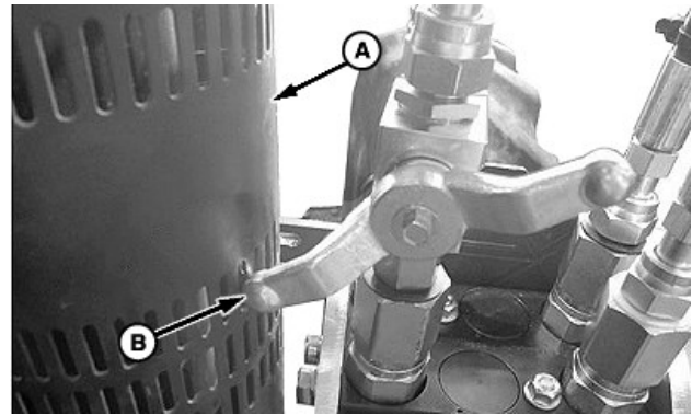
A—Exhaust Shroud B—Valve Handle
