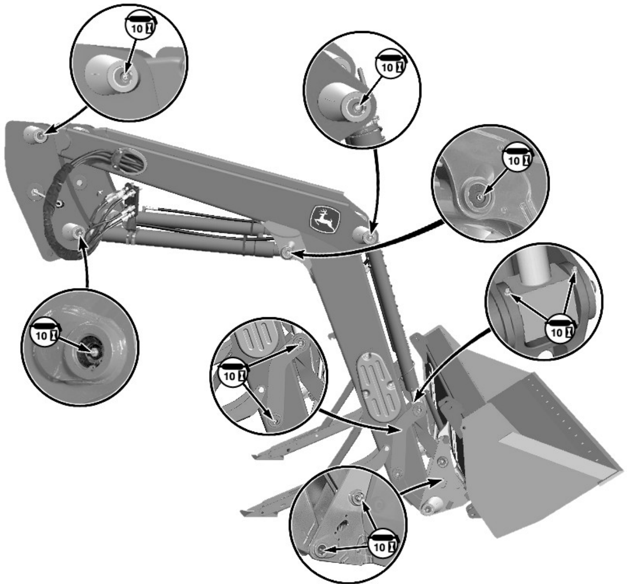
Lubrication Points
