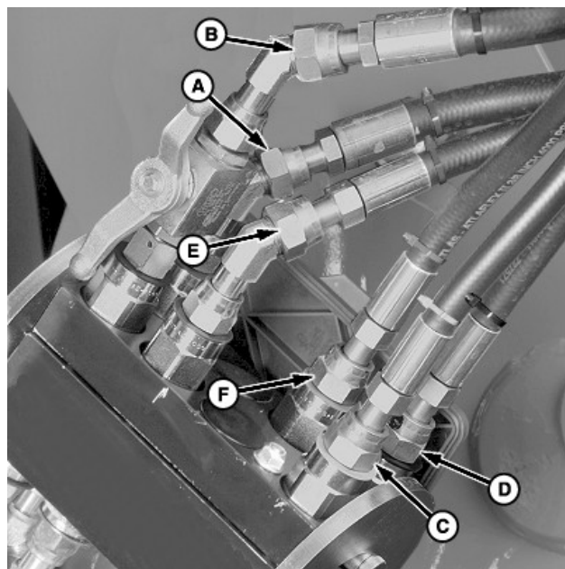
Multicoupler—Loader Half
