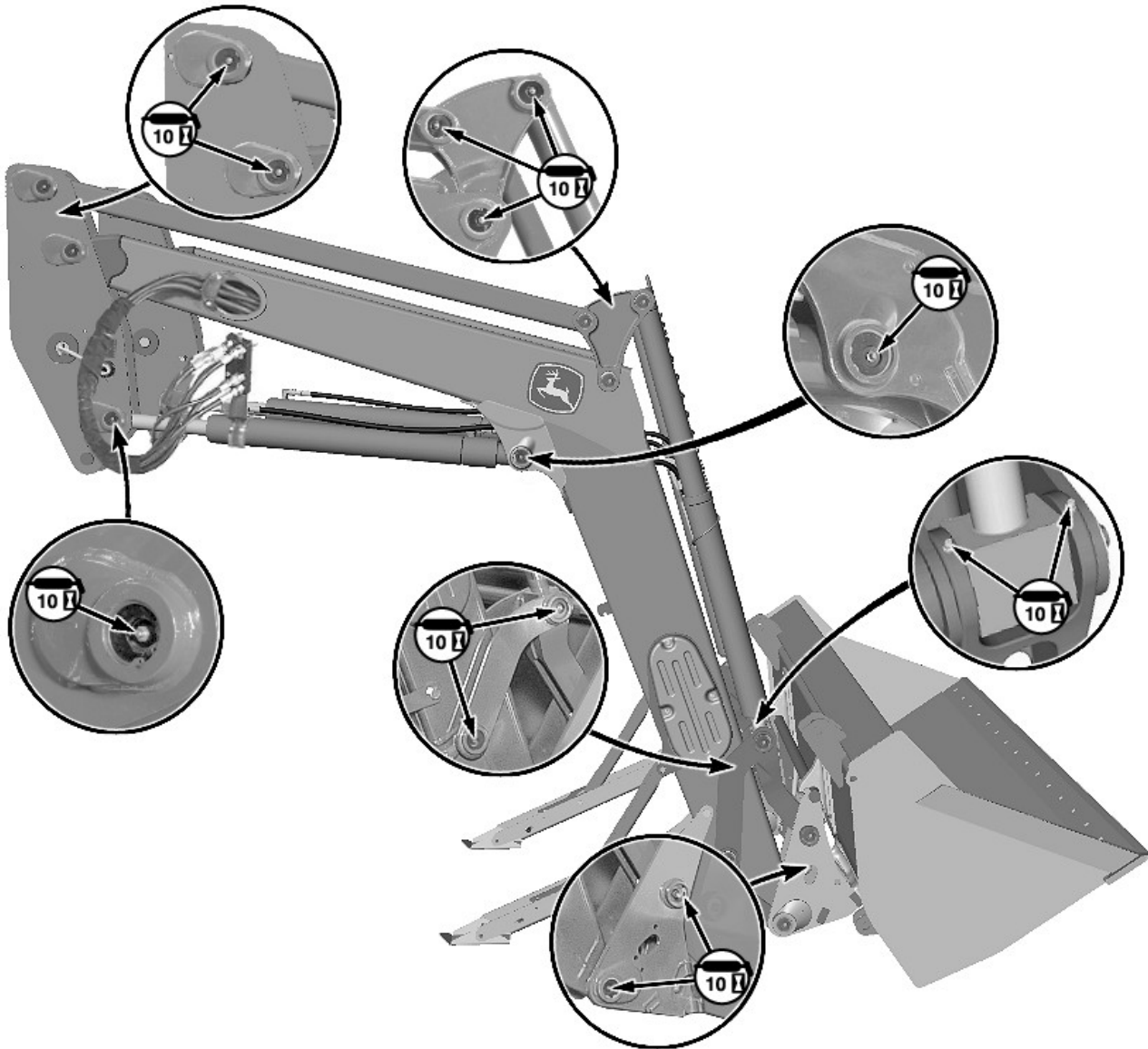
Lubrication Points
