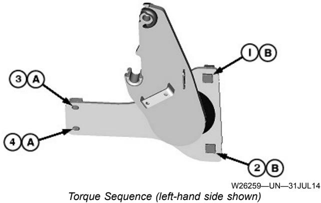
Torque Sequence (left-hand side shown)
