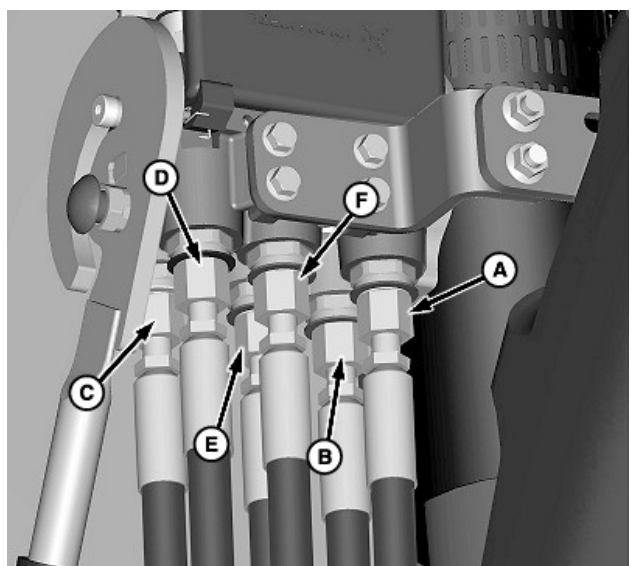
Multicoupler—Tractor Half
