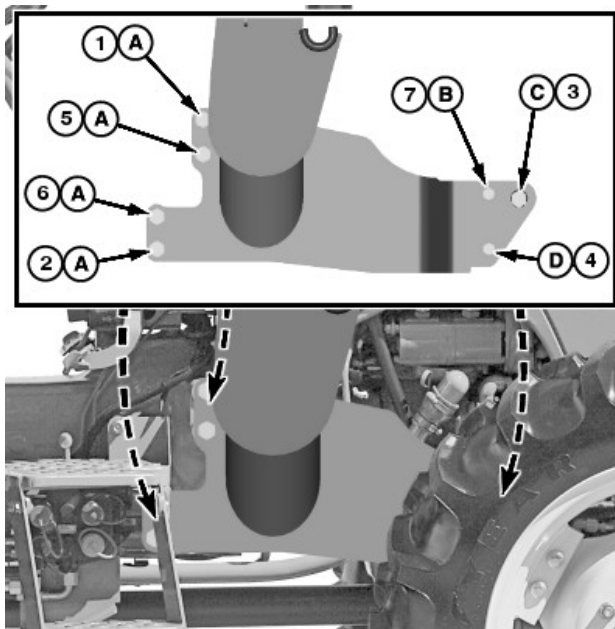
Torque Sequence (right-hand side shown)
