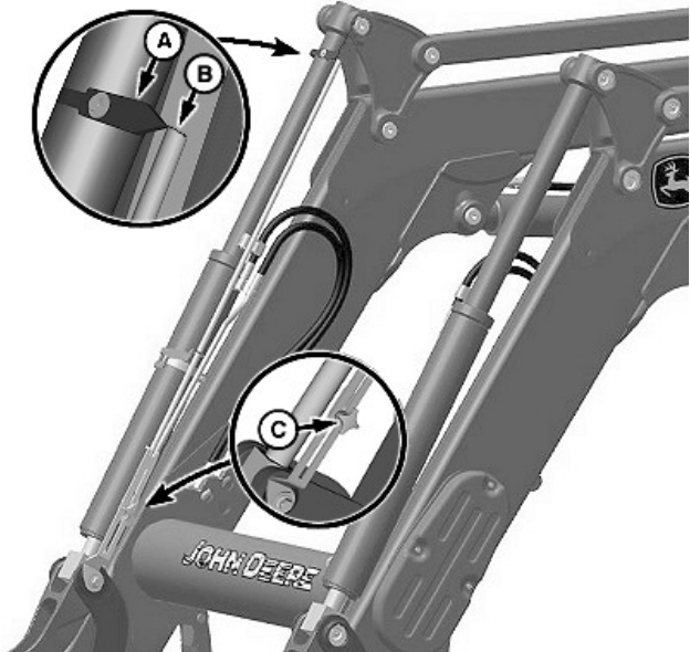
Mechanical Self-Leveling Loader
