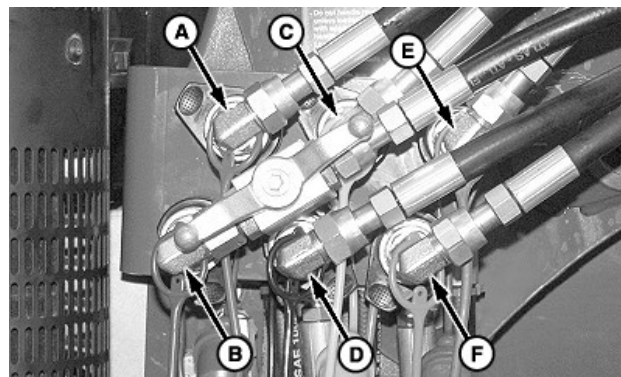
Mid-Mount Couplers
