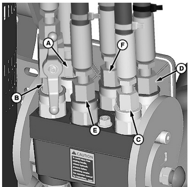
Multicoupler—Loader Half
