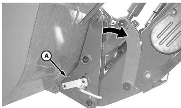
A—Carrier
