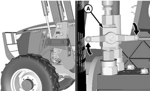
A—Handle, Shut Off Valve
