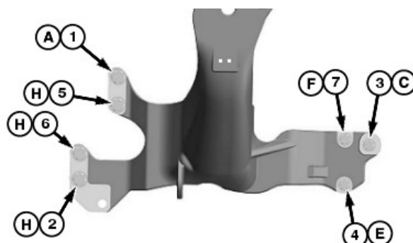
Torque Sequence—Right-Hand Side
