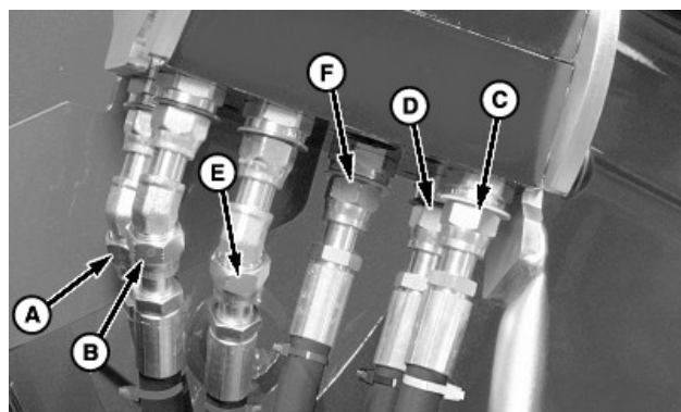
Multicoupler—Tractor Half
