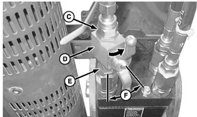
C—Hose Fitting D—Shutoff Valve E—Fitting F—Angle, 30—40 Degrees
