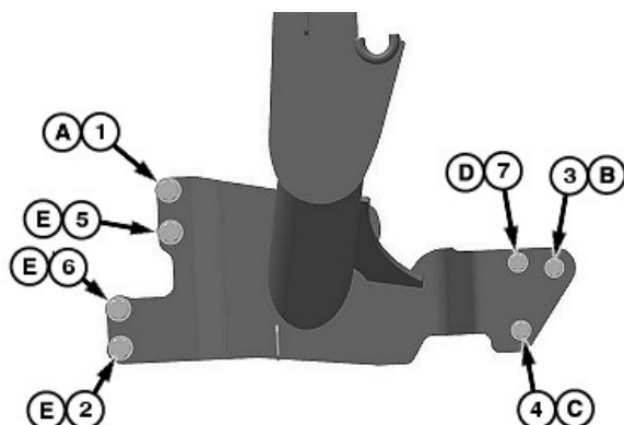
Torque Sequence (right-hand side)
