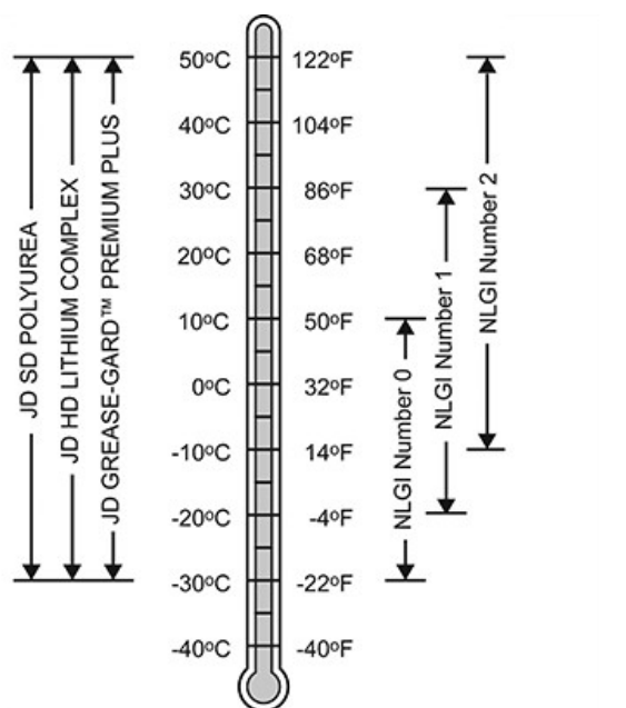
RG30199—UN—08MAR18 Greases for Air Temperature Ranges
