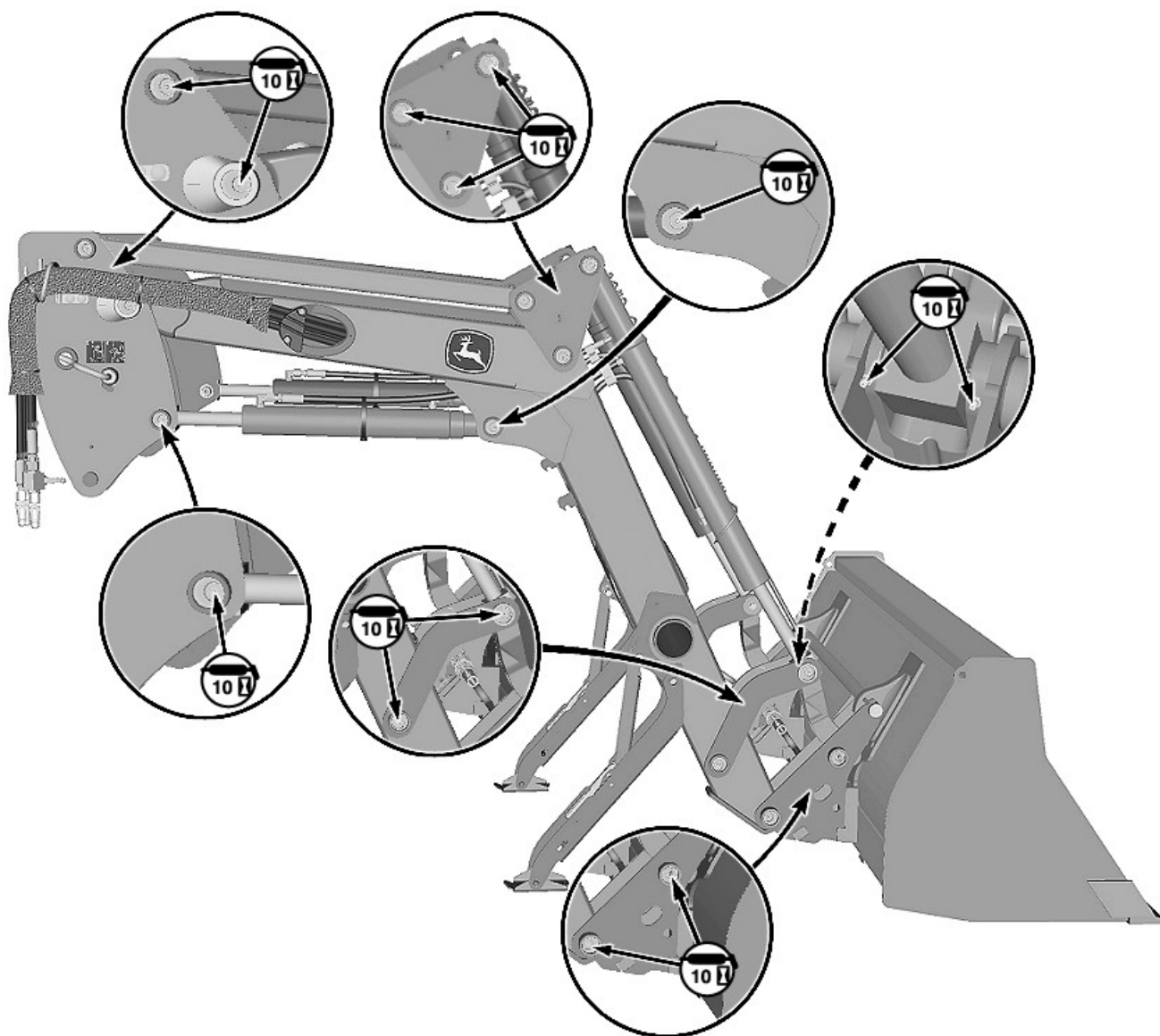
Lubrication Points
