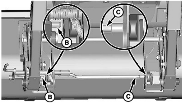
A—Handle B—Pin, Left-Hand Side C—Pin, Right-Hand Side
