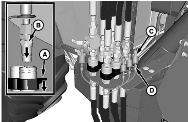
Raccords médians
