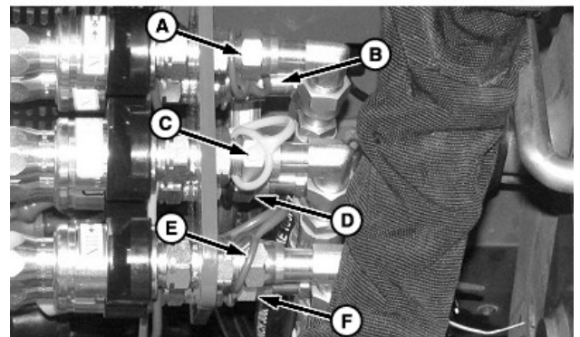
Hoses at Rear of Mid-Mount Couplers
