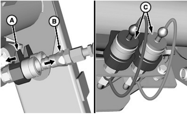
A—Coupler, Female B—Coupler, Male C—Plug (2 used)
