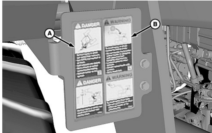
Toolbox Bracket—Left-Hand Side (5E series tractors)
