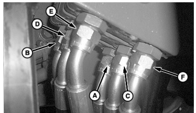
Hoses at Mid-Mount Valve
