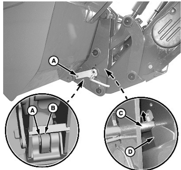
A—Pin (1 per side) B—Bracket, Attachment (1 per side)
