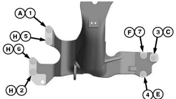
Torque Sequence—Right-Hand Side
