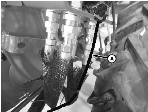
A—Harness, Three-Function (if equipped)
