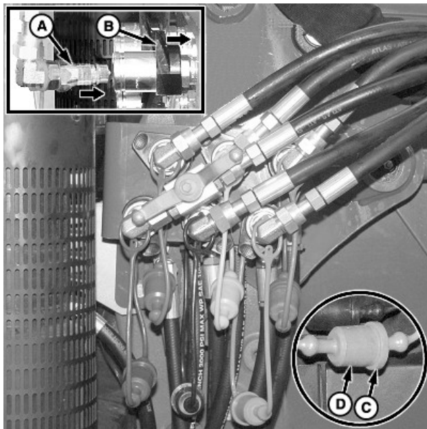
Mid-Mount Couplers
