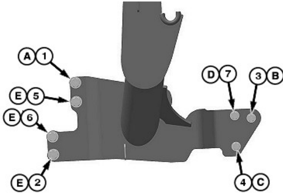
Torque Sequence (right-hand side)
