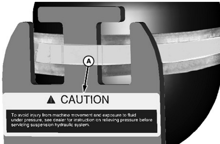
Accumulator for 520M Loader Suspension System
