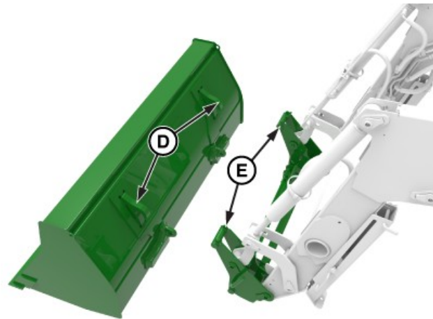
D—Hook (1 each side) E—Carrier Arm (1 each side)
