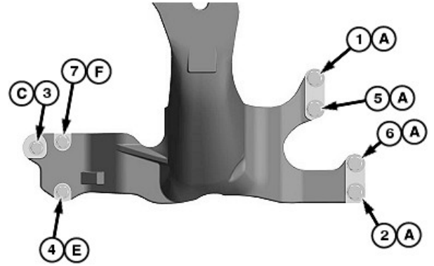
Torque Sequence—Left-Hand Side
