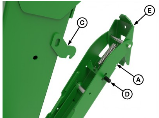
520M Parking Latch
