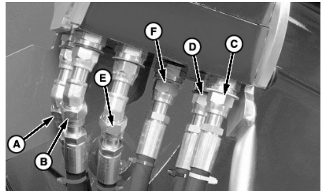
Multicoupler—Tractor Half
