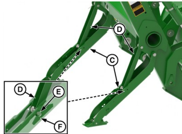
520M Parking Stand Shown
