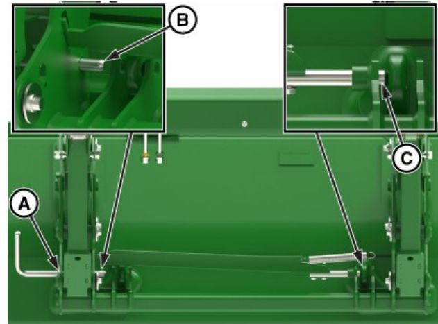
Latch Pins Retracted (Underside)
