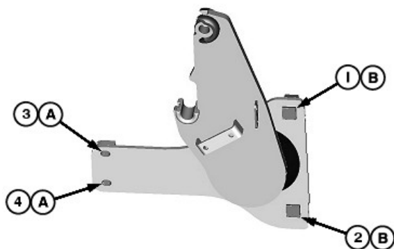
Torque Sequence (left-hand side shown)
