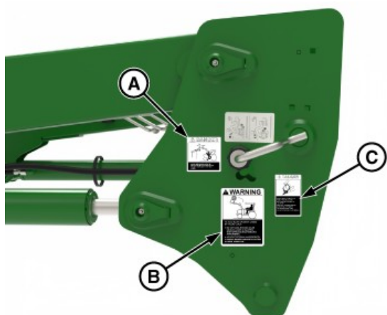
APY88262—UN—08DEC23 Left-Hand Side (520M NSL Shown)
