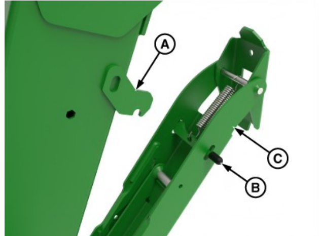
520M Parking Stand Shown
