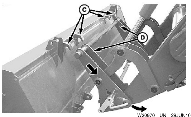
C—Hook (2 each side) D—Carrier Arm (1 each side)
