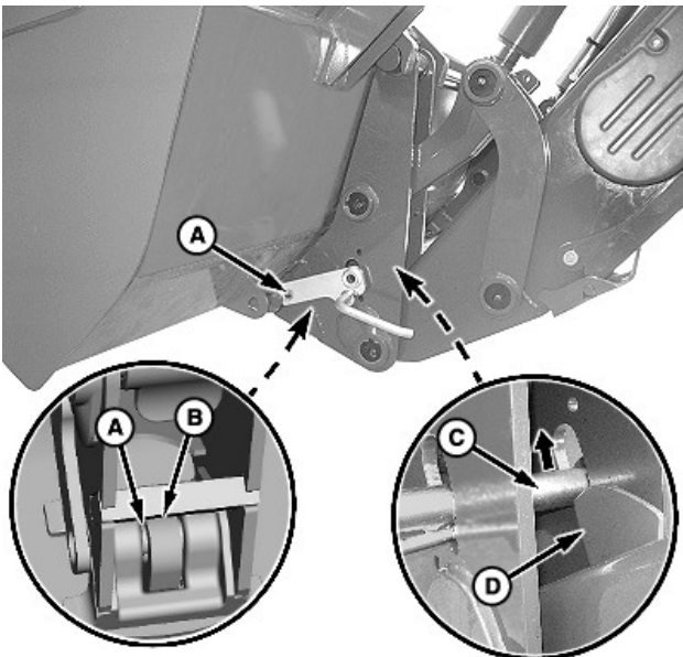
A—Pin (1 each side) B—Bracket, Attachment (1 each side)
