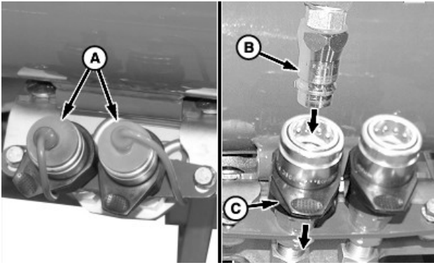
A—Plug (2 used) B—Coupler, Male C—Coupler, Female
