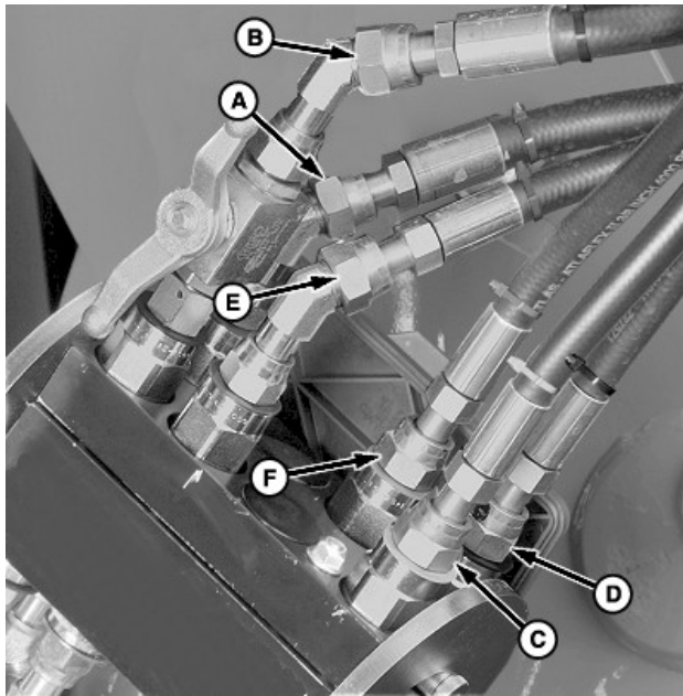
Multicoupler—Loader Half
