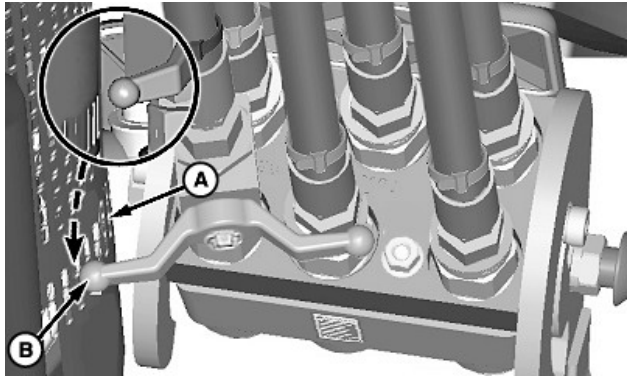
Valve Handle Clearance—Three-Function Shown
