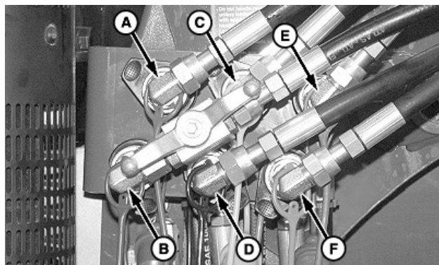
Mid-Mount Couplers
