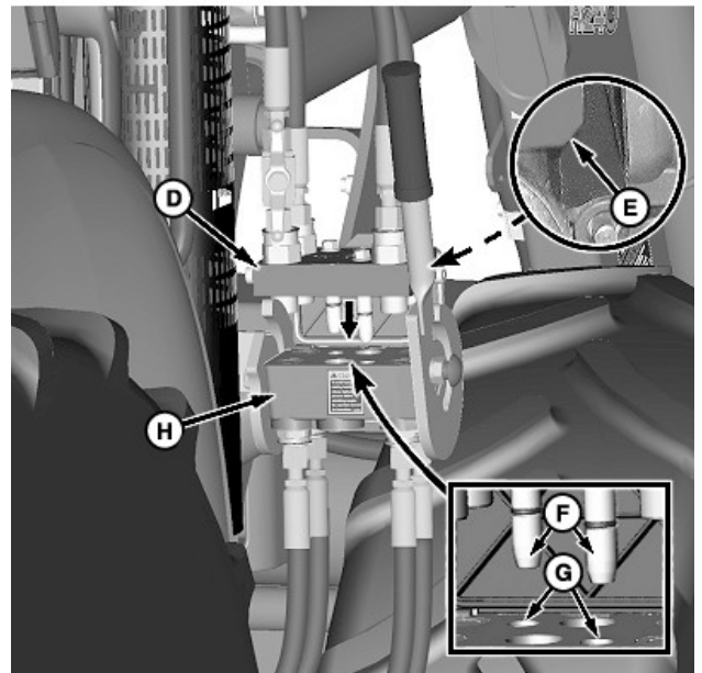
D—Coupler, Loader Half E—Chamfered Edge F—Locating Pin (2 used) G—Hole (2 used) H—Coupler, Tractor Half
