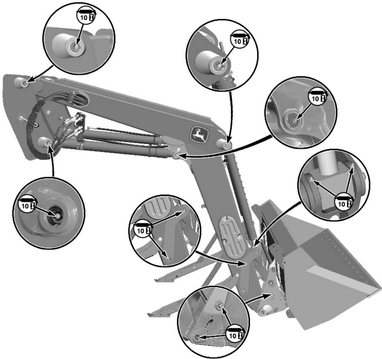
Lubrication Points
