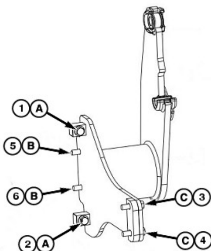
W28957—UN—03DEC20 Torque Sequence (left-hand side shown)
