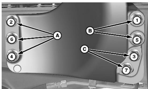
Torque Sequence (left-hand side shown)
