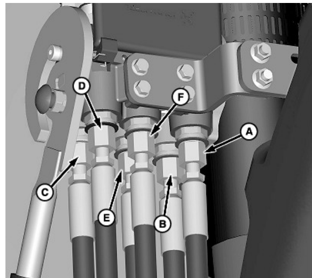
Multicoupler—Tractor Half
