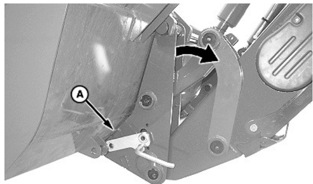
A—Carrier
