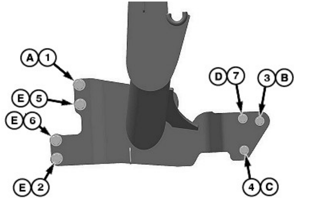
Torque Sequence (right-hand side)
