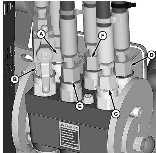
Multicoupler—Loader Half
