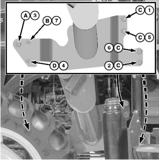
Torque Sequence (left-hand side shown)
