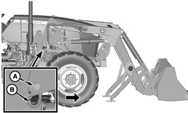
A—Pin (1 each side) B—Saddle (1 each side)
