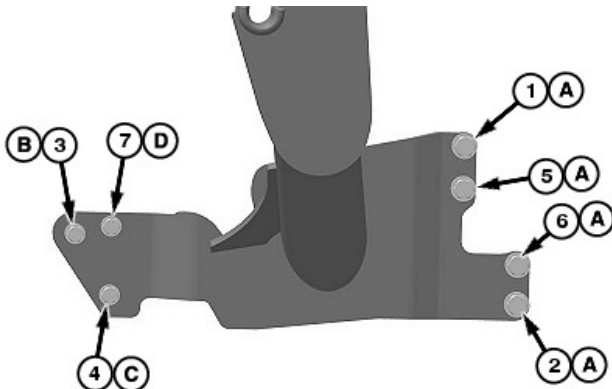
Torque Sequence (left-hand side)
