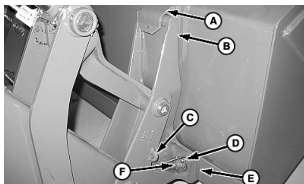
A—Hook (1 each side) B—Carrier C—Storage Position (1 each side) D—Pin, Quick Lock (1 each side) E—Strap (1 each side) F—Pin, Bucket (1 each side)
