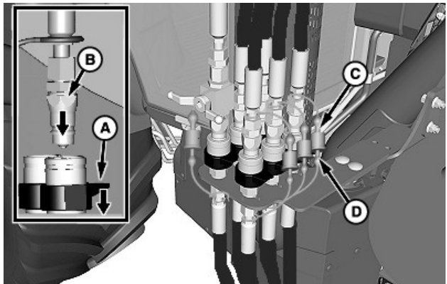
Mid-Mount Couplers
