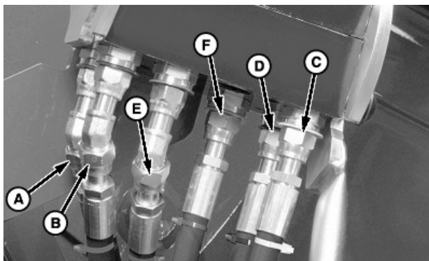
Multicoupler—Tractor Half
