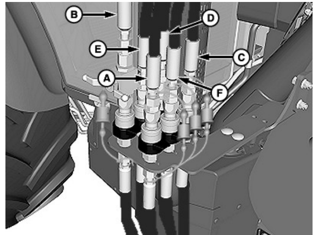
Mid-Mount Couplers
