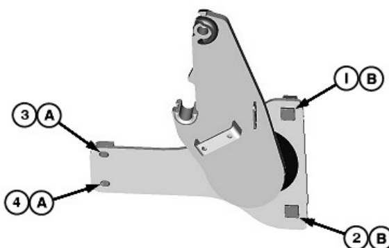
W26259—UN—31JUL14 Torque Sequence (left-hand side shown)
