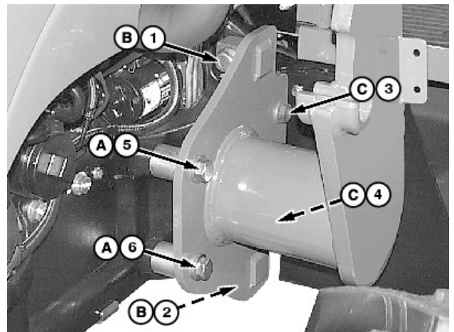
Torque Sequence (left-hand side shown)
