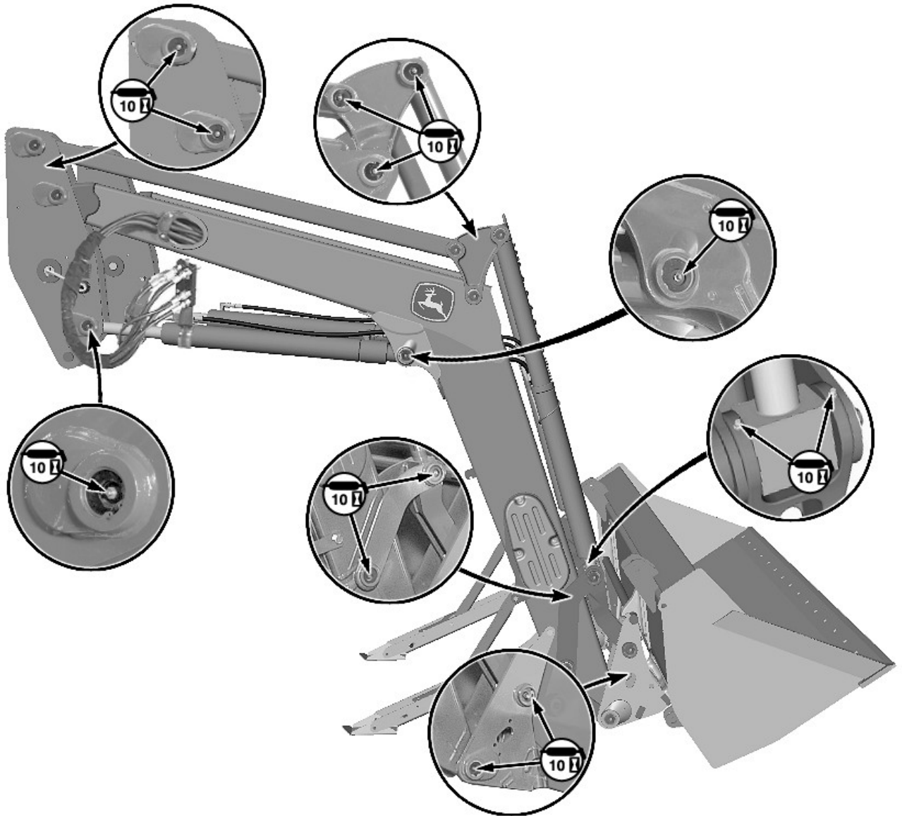
Lubrication Points
