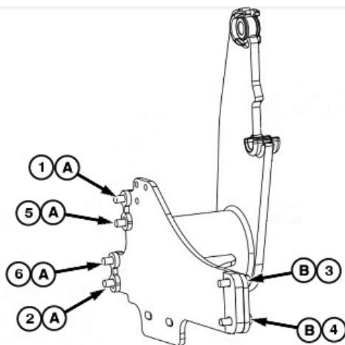
W28958—UN—03DEC20 Torque Sequence (left-hand side shown)
