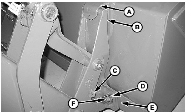
A—Hook (1 each side) B—Carrier C—Storage Position D—Quick-Lock Pin (1 each side) E—Carrier Strap (1 each side) F—Bucket Pin (1 each side)
