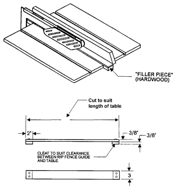
Figure 37 – Filler Piece
