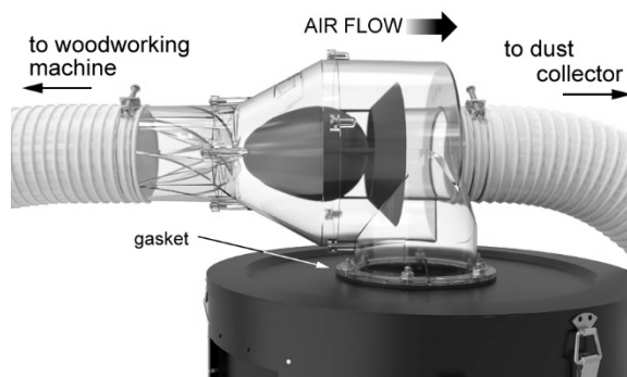
Figure 2: Hoses not provided; shown with JET bin
