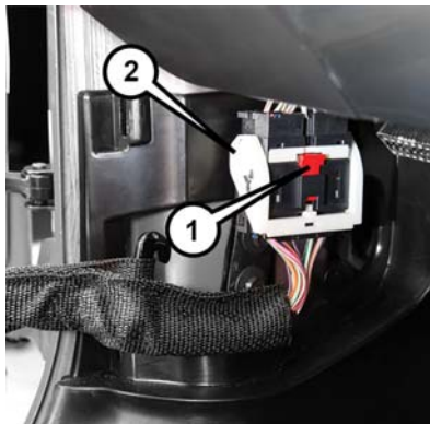
Closed Wiring Harness
